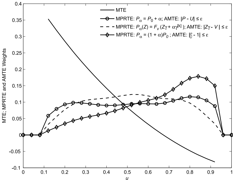
FIGURE 1.—Alternative definitions of the MPRT and the AMTE. This figure plots the marginal treatment effect ( MTE = E(Y_1 - Y_0 | X = x, U = u) ) and the marginal policy relevant treatment effect (MPRT) weights for three types of policy shifts: P_\alpha^A = P + \alpha , P_\alpha^B(Z) = F_V(Z\gamma + \alpha\gamma^{(k)}) , and P_\alpha^C = (1 + \alpha)P , where P is the probability of receiving treatment conditional on the observed covariates ( Z ). The equivalent definitions of the AMTE correspond, respectively, to the following three metrics for measuring the distance between P and U ( m(P, U) ): |P - U| , |Z\gamma - V| , and |\frac{P}{P_0} - 1| . The MTE, the MPRT, and the AMTE weights are evaluated at values of X such that E(Y_1 - Y_0 | X = x) = 0.13 . The average marginal policy effects are 0.1296 for the additive shift in P (A), 0.1274 for the additive shift in Z (B), and 0.0880 for the proportional shift in P (C). Estimated from NLSY data (see Carneiro, Heckman, and Vytlačil (2009), for details on estimating MTE).
