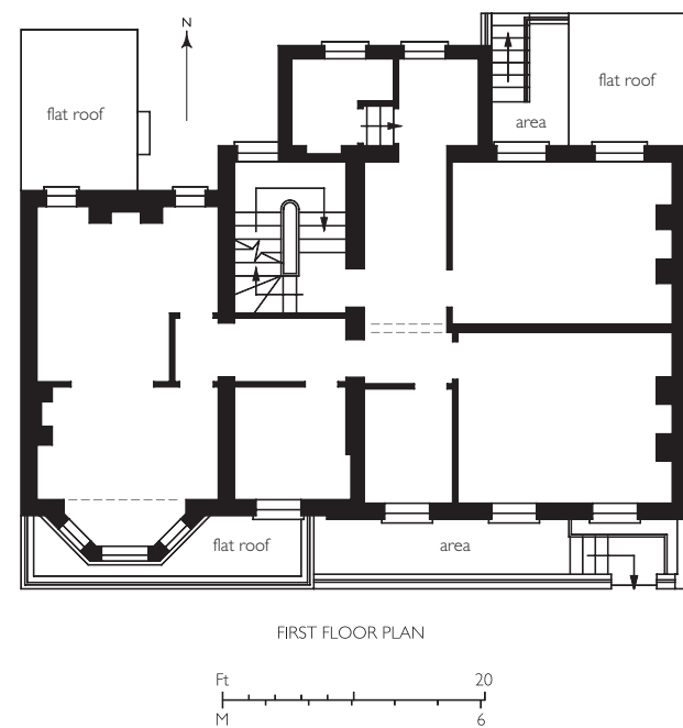
396. Hill House, 51–52 Hillreach, c.1815, enlarged to the west c.1845 and 1856–7. Plan (below) as subsequently altered, and (above) photograph of 2012
