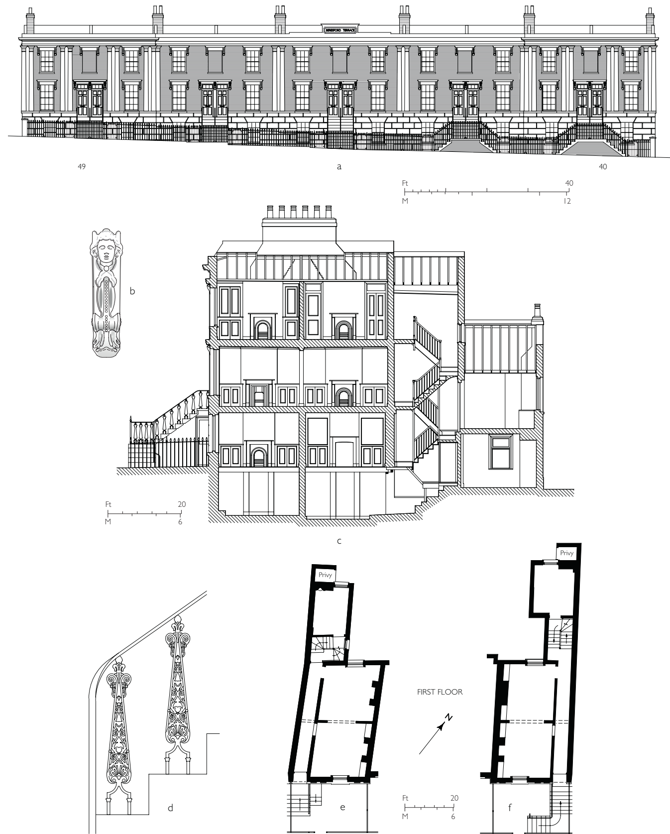
398. Beresford Terrace, 40-49 Hillreach, 1844-6: a south-east elevation; b mask bracket to door hood; c section through No. 41; d external staircase ironwork; e first-floor plan of No. 48; f first-floor plan of No. 41
