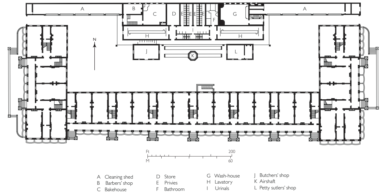
385. Marine Barracks, soldiers' quarters with service buildings to the rear, ground-floor plan as built 1844–5. Each large room housed twenty soldiers, each small room a married sergeant and family
