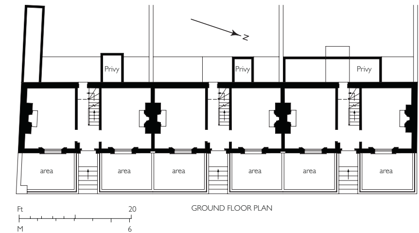
395. 106–110 Woodhill, plan as built
